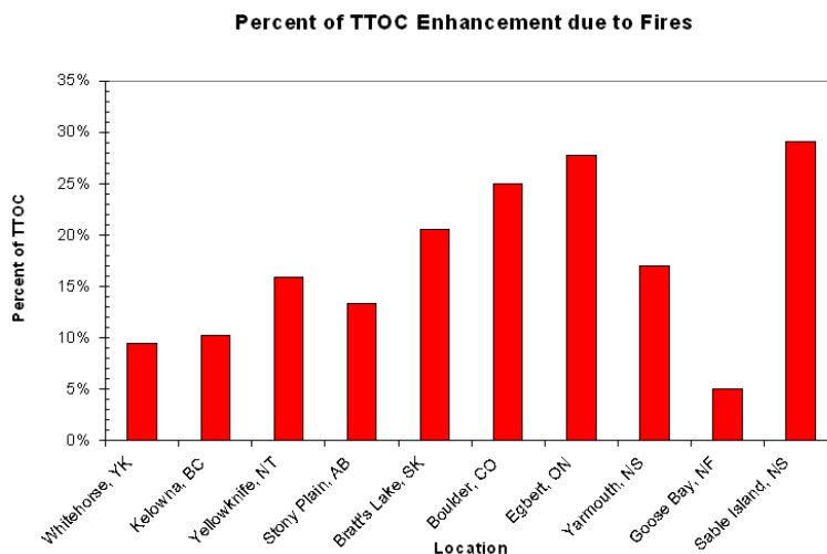
Figure 5. Percentage enhancement of Total Tropospheric Ozone Column (TTOC) due to boreal fires, at each of the summer ARC-IONS sites, estimated by the Lamina Identification (LID) method for each sounding [Thompson et al., 2007a,b], with additional ozone attributed by comparison of laminae with recent active fire exposure (according to NOAA/Hysplit trajectories) to background ozone. [from Luzik, 2009.]
