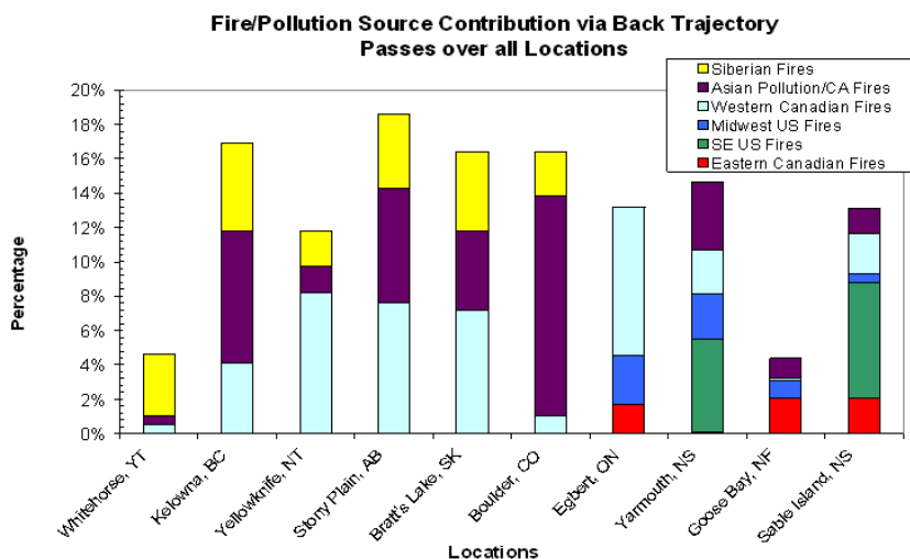
Figure 6. Attribution by geographical source region of percentage enhancement of Total Tropospheric Ozone Column (TTOC) due to boreal fires, at each of the summer ARC-IONS sites, estimated by NOAA/Hysplit backtrajectories. [From Luzik, 2009.]
