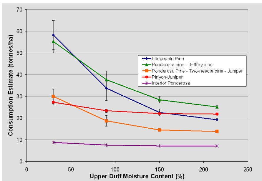
Figure 3. Fuel consumption is quantified with the US Forest Service’s CONSUME model based on fuel type and condition. The graph shows emissions as a function of upper duff moisture – as a percentage of dry mass. Similar data has been collected by the Canadian Forest Service for their CanFIRE model. Using field-measured fuel conditions and the resulting fuel consumption after the burn, relationships between the forest type and moisture conditions are developed to determine fuel consumption and emission of carbon-based gas (CO 2 , CO, and hydrocarbons including methane).
