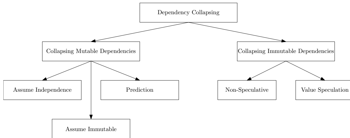
Figure 2.9: Dependency Collapsing
