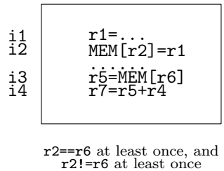
Figure 2.12: Memory Cloaking
